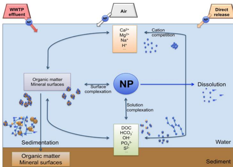
Figure 3: Physicochemical transformation of NPs when released into the aquatic environment (Vale et al., 2016)
