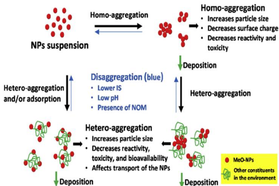
Figure 2: Common physical transformations that MeO-NPs undergo in the aquatic environment (Amade et al., 2017)
