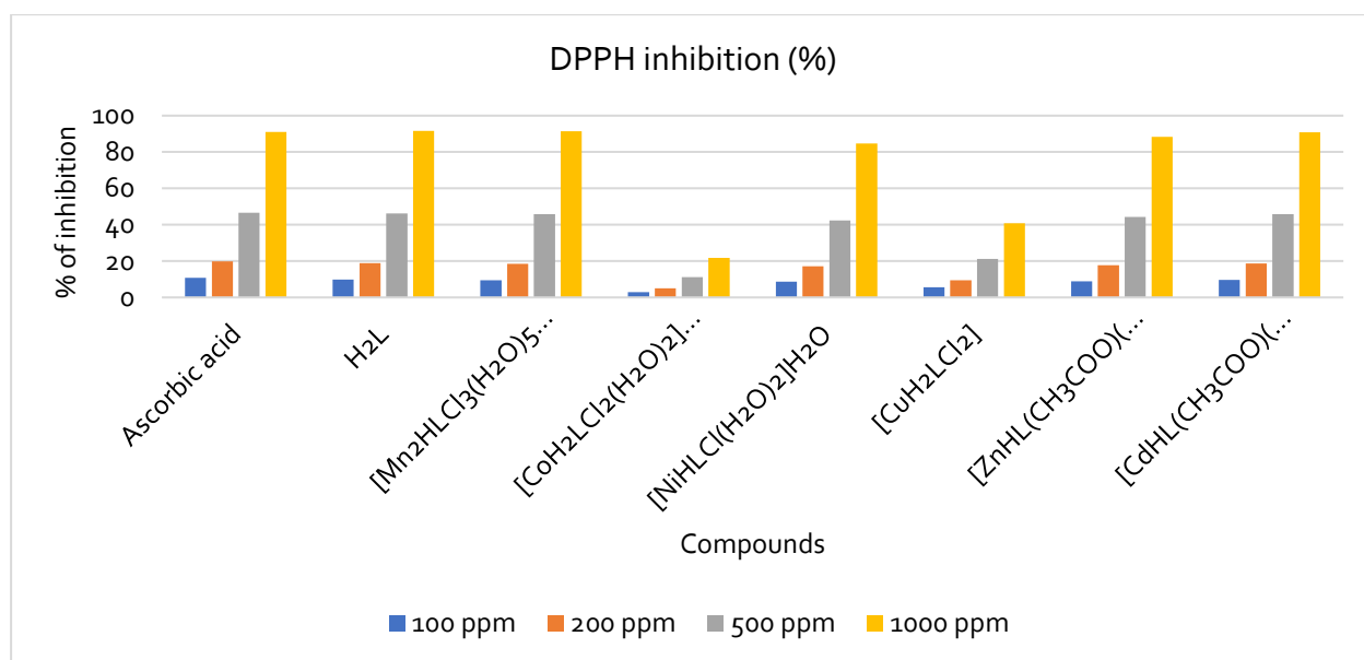
Figure 19. The DPPH free radical scavenging activity of compounds
