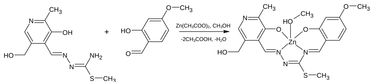
Figure 11. Synthesis of Zn(II) complex.
