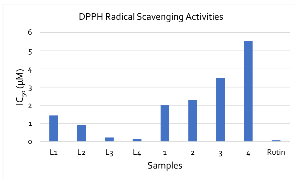
Figure 18. The radical scavenging activities of assayed compounds
